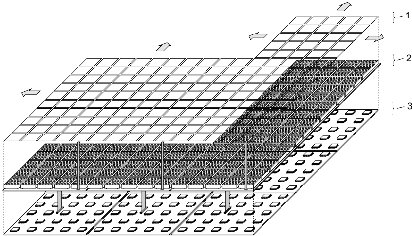
Fig. 7. The BioWall, a reconfigurable and completely scalable tissue capable of interacting with its environment by means of a large number of touch-sensitive elements (1) coupled with two-color dot LED displays (2) and reconfigurable circuits (3).
