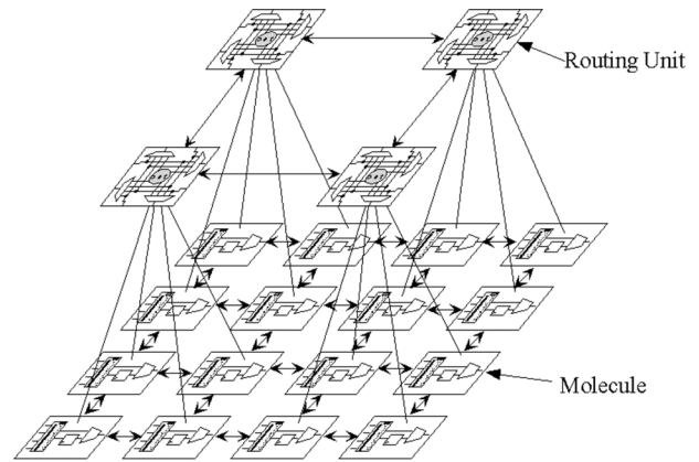
Fig. 4. Molecules and routing units.
