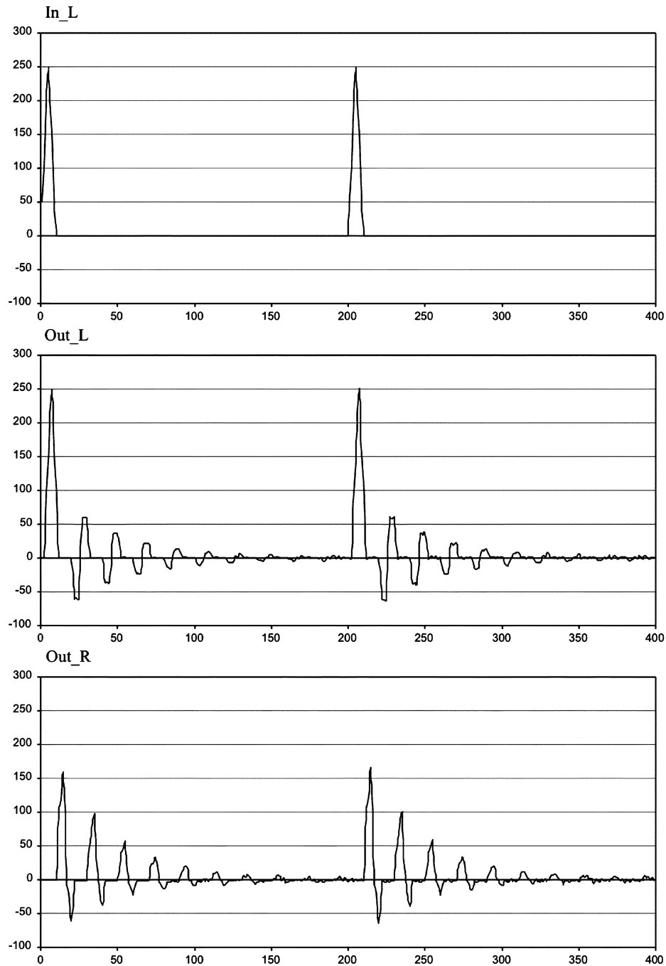
Fig. 19. Cell output in response to pulses applied to one input.
