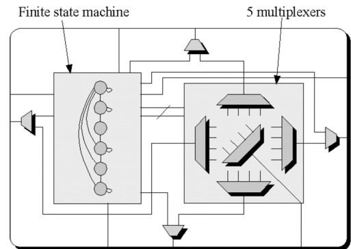
Fig. 5. Routing unit.
