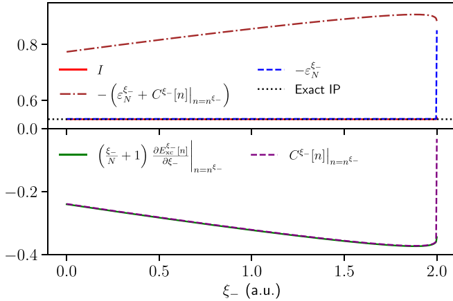
FIG. 2. The exact KS HOMO energy ( \epsilon_N^{\xi_-} ) is minus the exact IP for 0 \leq \xi_- < \frac{N}{N-1} . Each term of Eq. (7) is shown. The calculation of I via Eq. (7) equals the exact IP for all \xi_- as expected. We choose v_s^{\xi_-}(x) to asymptotically approach 0.
