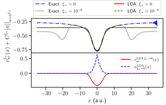
FIG. 9. The LDA xc potential as \xi_+ \rightarrow 0^+ and \xi_+ = 0 . The LDA xc potential does not visibly change as \xi_+ \rightarrow 0 . The exact potential is shown for reference.
