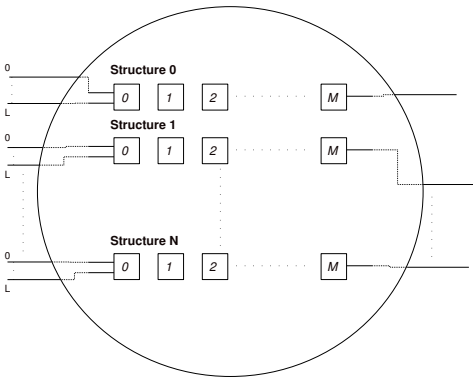
Fig. 1. The structural part of a cell: a cell can have N independent structures that can be formed of M components (gates, MUXes, CLBs, etc.). Each structure is allocated L inputs and 1 output by the cell where they can connect outside. A structure can not connect to another structure within the cell.
