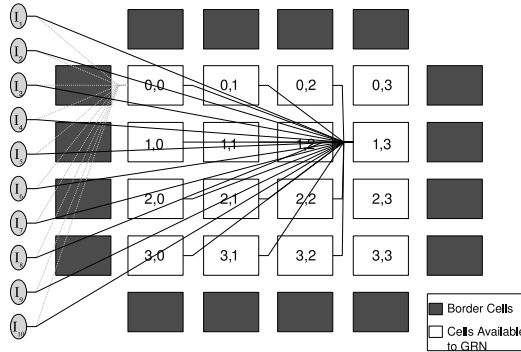
Fig. 5. An example 4 \times 4 organism with 10 inputs is shown. The available structural connections for cells 0,0 ; 0,1 and 1,3 are drawn to illustrate how the cells can connect to form a CGP circuit.
