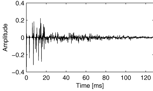
Fig. 4. The echo impulse response that is used in all the simulations.
