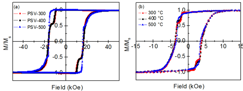
FIG. 1. (Color online) Hysteresis loops of (a) simulated and (b) experimentally fabricated FePt/Ag/FePt PSVs with varying Ag post-annealing temperatures of 300, 400, and 500 °C.
