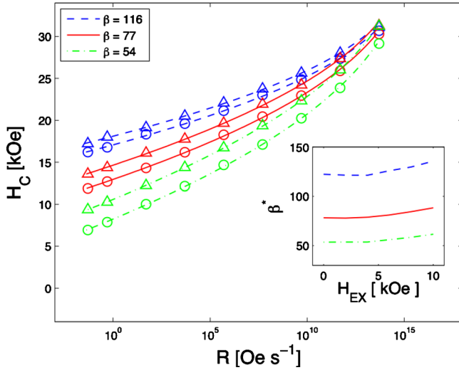
FIG. 1. (Color online) Dependence of the coercive field H_C on the external field sweep rate R for different thermal stability factors for the noninteracting case ( \circ ) and the case with dipolar interactions and exchange H_{EX}=10 kOe ( \Delta ). Lines represent the least-square fits of Eq. (3). Inset: Dependence of \beta^* obtained from fitting Eq. (3) for 0 \leq H_{EX} \leq 10 kOe.
