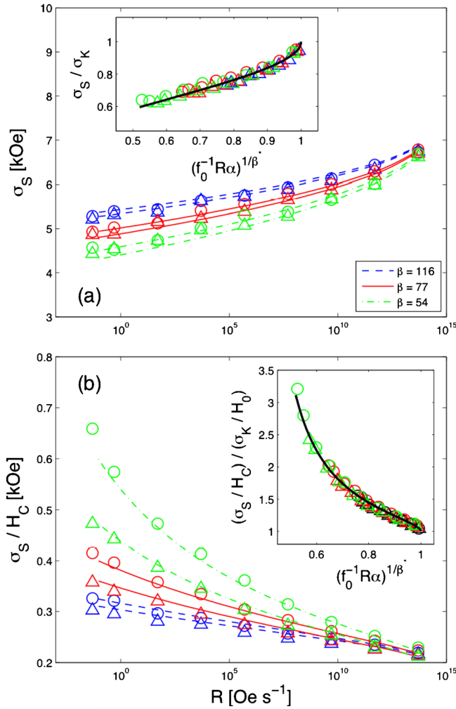
FIG. 2. (Color online) (a) Dependence of the switching field distribution width \sigma_S on the external field sweep rate R for different thermal stability factors for the non-interacting case ( \circ ) and the case with dipolar interactions and exchange H_{EX}=10 kOe ( \Delta ). Lines represent plots of Eq. (4) using H_0 and \beta^* obtained from fitting Eq. (3) to H_C(R) . Inset: A collapse of all the fitted curves onto a universal function y=1-2^{-1}[\ln(1/x)]^{1/2} after rescaling the axes. \alpha=2\beta^*(1-H_C/H_0)/H_0 . (b) The same as (a) but for the ratio \sigma_S/H_C given by Eq. (5). Inset: the universal function has now the following form: y=\{1-2^{-1}[\ln(1/x)]^{1/2}\}/\{1-[\ln(1/x)]^{1/2}\} .
