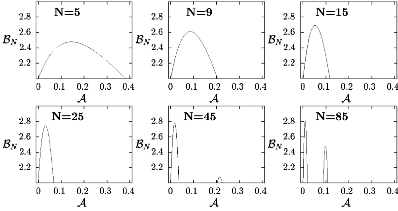
FIG. 2. Maximum violations of the inequality |\mathcal{B}_N| \leq 2 imposed by local realistic theories in the limit of large squeezing. \mathcal{B}_N is plotted as a function of \mathcal{A} \equiv \mathcal{J}e^{+2r} for different N .
