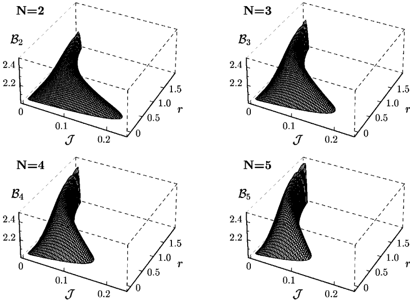
FIG. 1. Violations of the inequality |\mathcal{B}_N| \leq 2 imposed by local realistic theories with the entangled two-mode EPR ( N=2 , as in Ref. [8]), three-mode GHZ ( N=3 ), four-mode GHZ ( N=4 ), and five-mode GHZ ( N=5 ) states.
