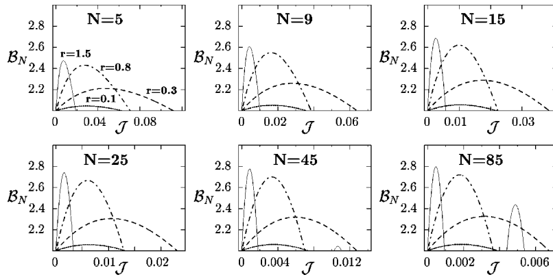
FIG. 3. Violations of the inequality |\mathcal{B}_N| \leq 2 imposed by local realistic theories for different N at certain amounts of squeezing of the N -mode GHZ states: r=0.1 ( \approx 0.9 dB), r=0.3 ( \approx 2.6 dB), r=0.8 ( \approx 6.9 dB), and r=1.5 ( \approx 13 dB). \mathcal{B}_N is plotted as a function of \mathcal{J} . Note that the axes of the displacement parameter \mathcal{J} vary in scale. The larger N becomes, the smaller become the displacements required.
