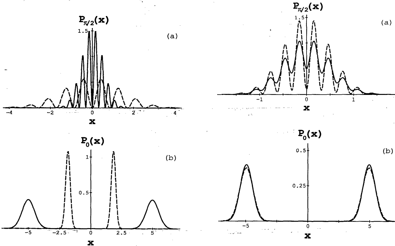
FIG. 2. Effect of damping for a scaled time \tau = \Gamma t = 0.02 . Plots of the homodyne statistics of (a) P_{\pi/2}(x) and (b) P_0(x) vs x for the damped versions of the states f(|5\rangle - |-5\rangle) (solid line) and f\hat{S}(-1,0)(|5\rangle - |-5\rangle) (dashed line). The dashed plots have been scaled by the factors e^{\pm 1} so as to coincide with the scales of the solid line plots.
