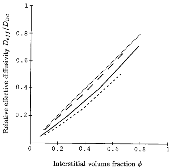
FIGURE 4 Effect of elongating (aligned) cells on effective diffusivity. Solid curve: cubic cells (1:1:1); long dashes: cells elongated (5:1:1) in direction of diffusion; short dashes: cells elongated (1:5:1) perpendicular to direction of diffusion; dotted line: upper bound D_{\text{eff}}/D_{\text{int}} = \phi .
