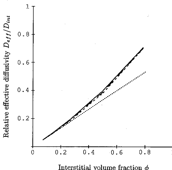
FIGURE 3 Effective diffusivity as a function of interstitial volume fraction: comparison of aligned, staggered, and doubly staggered cases. Solid curve: aligned; long dashes: staggered in one direction; short dashes: staggered in two directions; dotted line: D_{\text{eff}}/D_{\text{int}} = (2/3)\phi approximation for small \phi (aligned).
