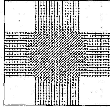
Fig. 5 Magnetization configurations of a cross-junction in the equilibrium state for the network structure with s=0.5 \mu\text{m} .
