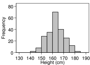
Heights of 222 women admitted to the VenUS I trial.
