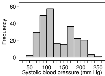
Systolic blood pressure in 251 patients admitted to an intensive therapy unit.
