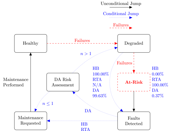
Fig. 6. Figure showing the flow of actions that are taken for DSR1
