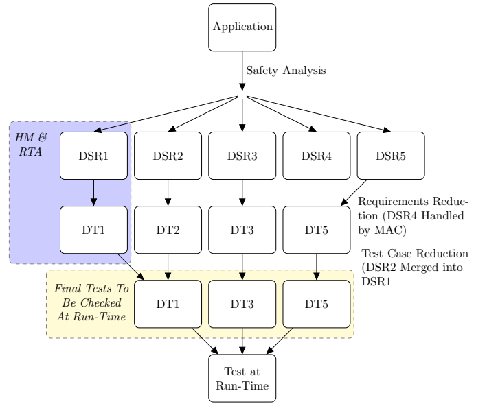
Fig. 1. Figure showing the generation of the Dependability Tests
