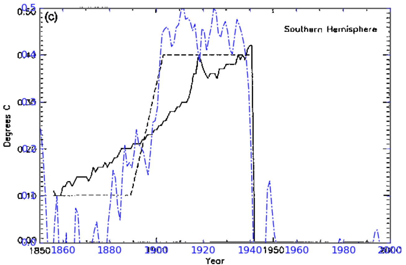
Figure 19 of Folland et al (1995) (in black), showing the HadSST bucket correction (solid line), and an estimate of the bucket bias from coastal weather stations determined by Jones et al (1991). The blue dashed line overlaid on the figure is our (global) estimate of the bucket bias using a larger set of coastal weather stations, which shows a similar profile back to about 1880.
