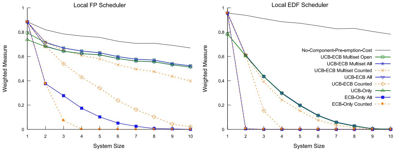
Figure 10 - Varying the system size from 1 to 10. An increase of 1 in the system size relates to introducing another component that brings along with it another 5 tasks and an increase in the cache utilisation of 2.
