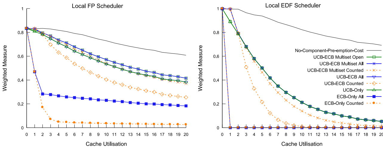
Figure 12 - Varying the cache utilisation from 0 to 20
