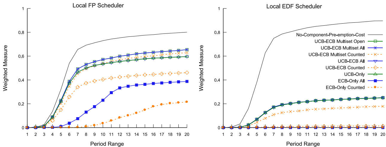
Figure 14 - Varying the period range of tasks from [1, 100]ms to [20, 2000]ms (while fixing the server period at 5ms)
