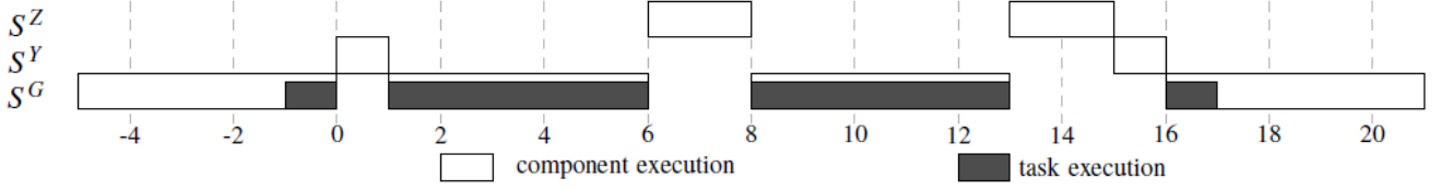
Figure 2 - Example global schedule to illustrate the server suspend and resume calculation with P^G = P^Z = P^Y = 8 , Q^G = 5 , Q^Z = 2 , Q^Y = 1 .
