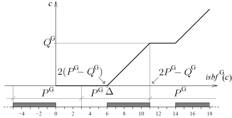
Figure 1 - General case of a server where Q^G = 5 and P^G = 8 showing it can take up to 6 time units before a task receives supply
