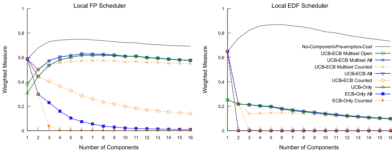
Figure 9 - Varying the number of components from 1 to 16, while keeping the number of tasks in the system fixed
