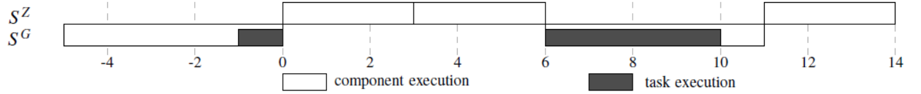
Figure 3 - Example global schedule to illustrate the disruptive execution calculation with P^G = P^Z = 8 , Q^G = 5 , Q^Z = 3 .
