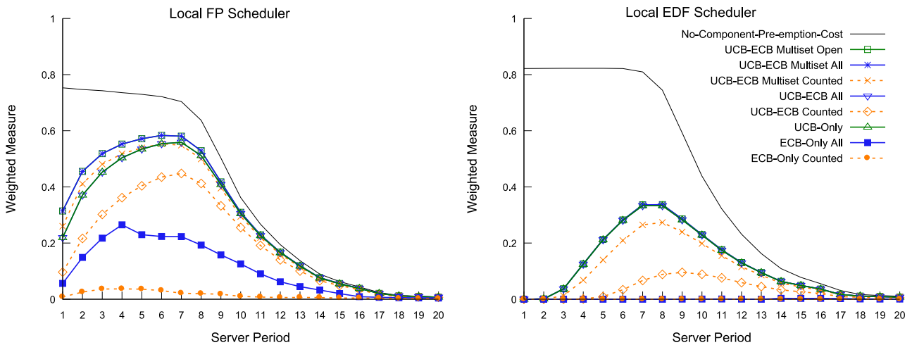
Figure 11 - Varying the server period from 1ms to 20ms (fixed task period range of 10ms to 1000ms)
