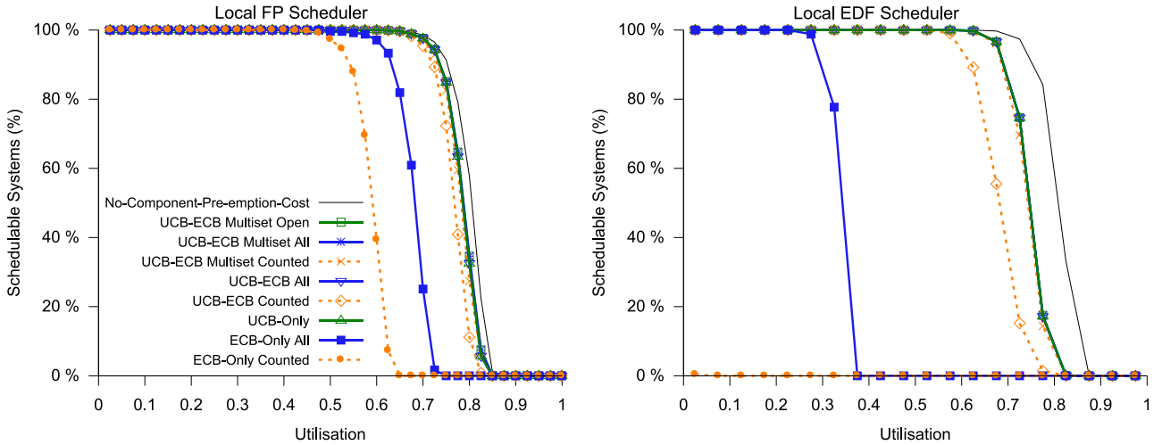
Figure 6 - Percentage of schedulable tasksets at each utilisation level for the case study tasks
