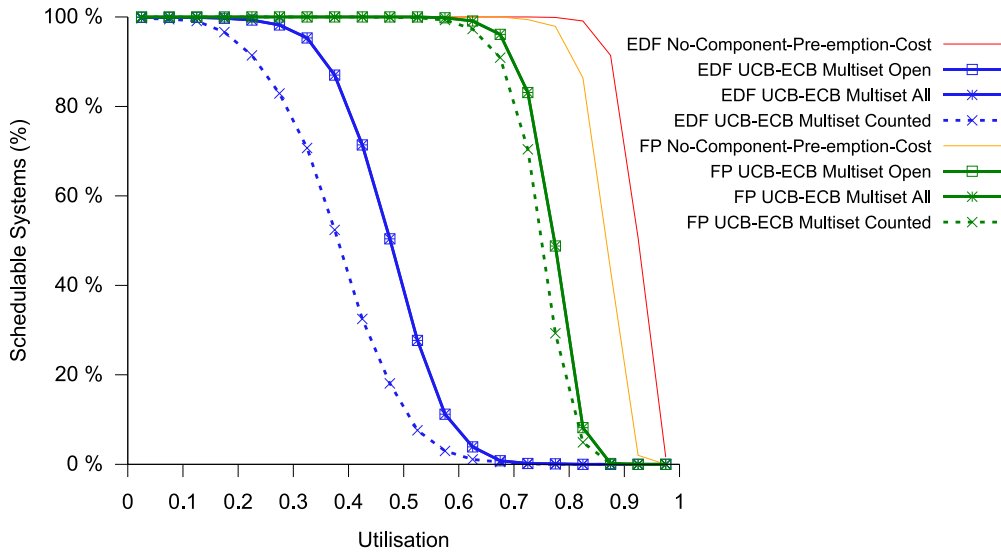
Figure 8 - Percentage of schedulable tasksets at each utilisation level for the synthetic tasksets directly comparing the analysis for local FP and EDF schedulers
