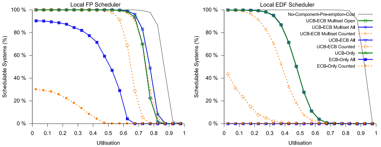
Figure 7 - Percentage of schedulable tasksets at each utilisation level for the synthetic tasksets
