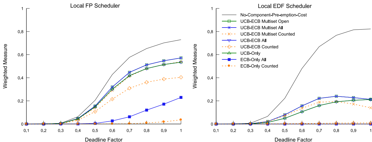
Figure 16 - Varying the task deadlines via D_i = xT_i by varying x from 1 to 0.1 in steps of 0.1
