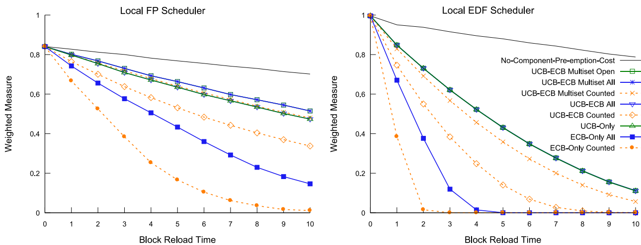
Figure 15 - Varying the block reload time (BRT) from 0 to 10 in steps of 1
