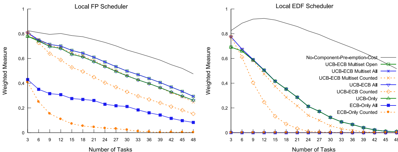
Figure 13 - Varying the total number of tasks from 3 to 48 (1 to 16 tasks per component)
