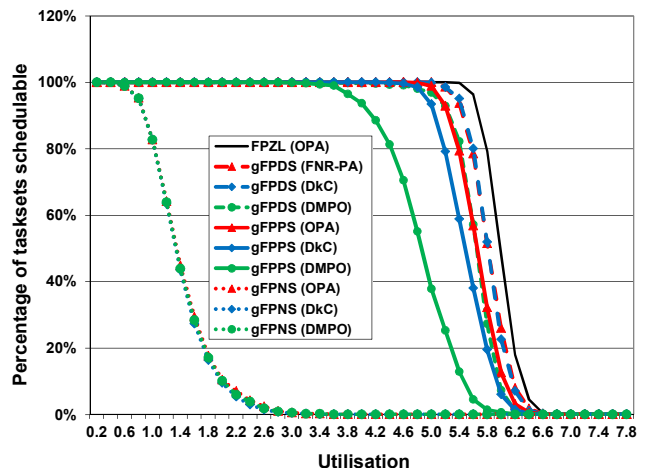
Figure 4: Success ratio for m = 8 , n = 40 , implicit deadlines
