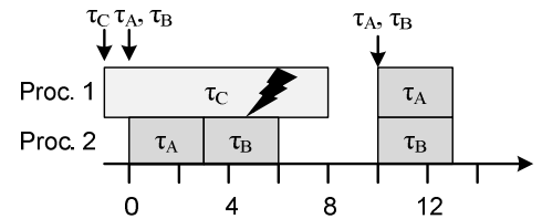
Figure 3: Schedule with gFPNS.
